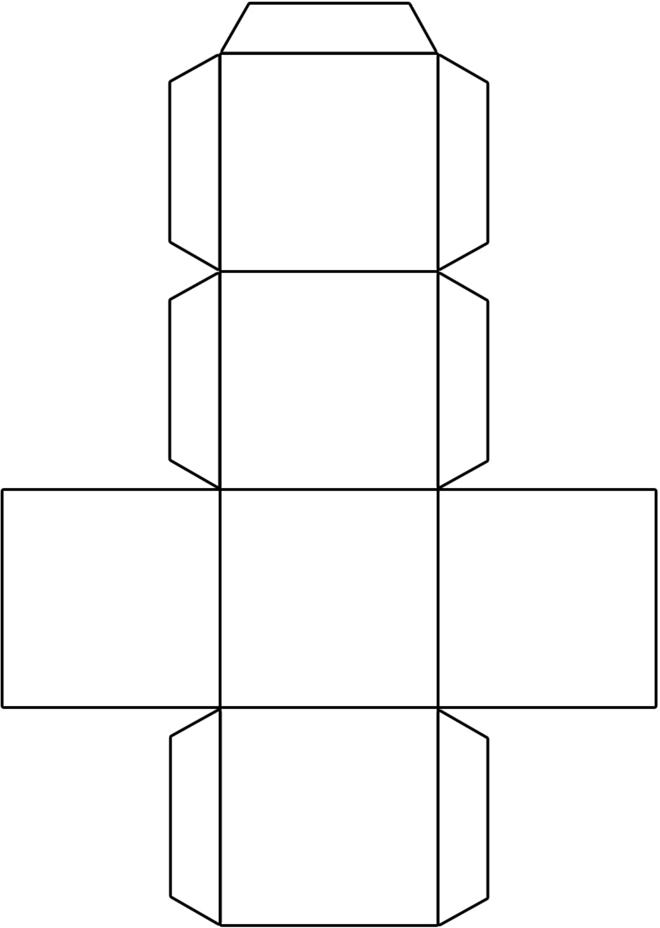
Hexahedron (platonic solid)
